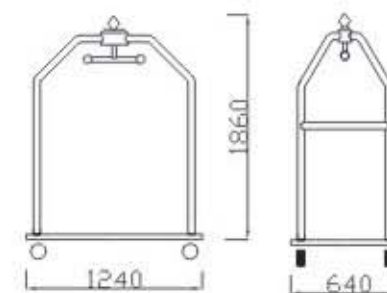
91.2005A Dimension
