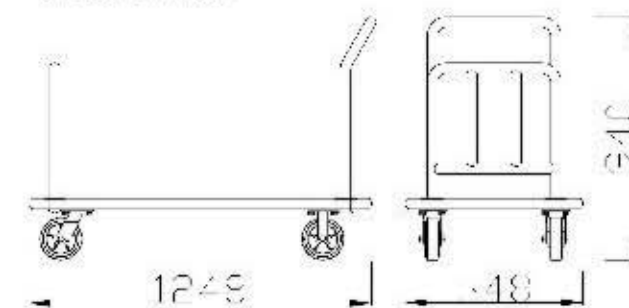
91.2008A Dimension
