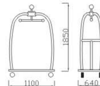
91.2111A Dimension
